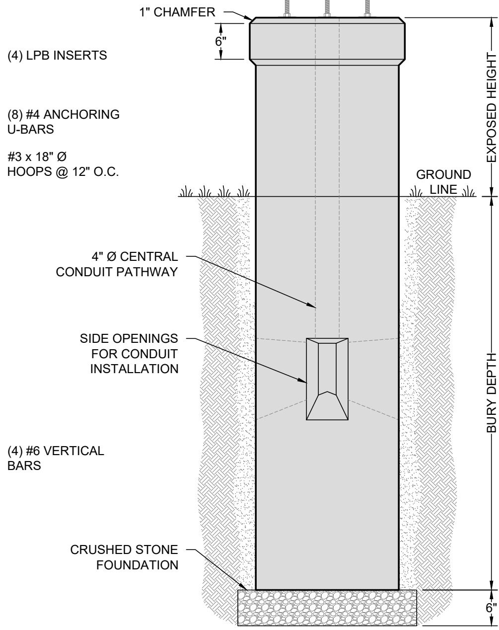
INSTALLED PRODUCT VIEW SCALE: 3/4" = 1'-0"
